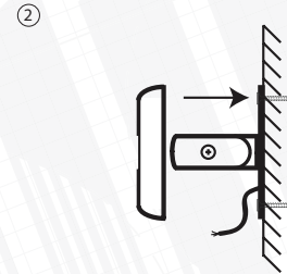
② Fix the loudspeaker bracket on the wall with fasteners suitable for your wall type. Place decorative cover on the bracket.
