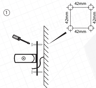
① Drill four holes according to the drawing. Distance between the mounting points - 42 mm.
