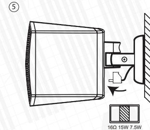
⑤ Connect Phoenix connector to socket. Set the desired loudspeaker power tap.
